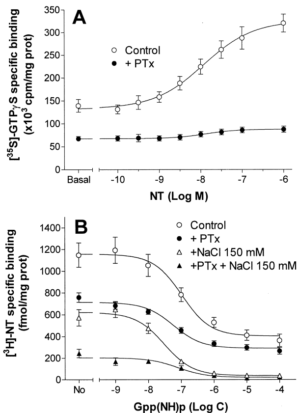
Fig. 1. (A) NT-induced [ ^{35} S]GTP \gamma S binding on homogenates from CHO-NTR cells previously treated in the presence (closed symbols) or in the absence (open symbols) of PTx (100 \mu g/ml, 20 h). (B) Effect of Gpp(NH)p (increasing concentrations) and NaCl (control, circles; 150 mM NaCl, triangles) on the specific binding of [ ^3 H]NT to homogenates from CHO-NTR cells previously treated in the presence (closed symbols) in the absence (open symbols) of PTx (100 \mu g/ml, 20 h). Data shown are mean \pm S.D. from five (A) and three (B) different experiments performed in duplicate, respectively.
